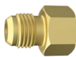
170901 Amarelo Rosca Externa: TC 1/2" TERMINAL BSP X TC Rosca Interna: BSP 3/8"
