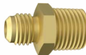
170402 Amarelo NIPLÉ TC X NPT Rosca Externa: TC 3/8" Rosca Externa: NPT 1/2"
